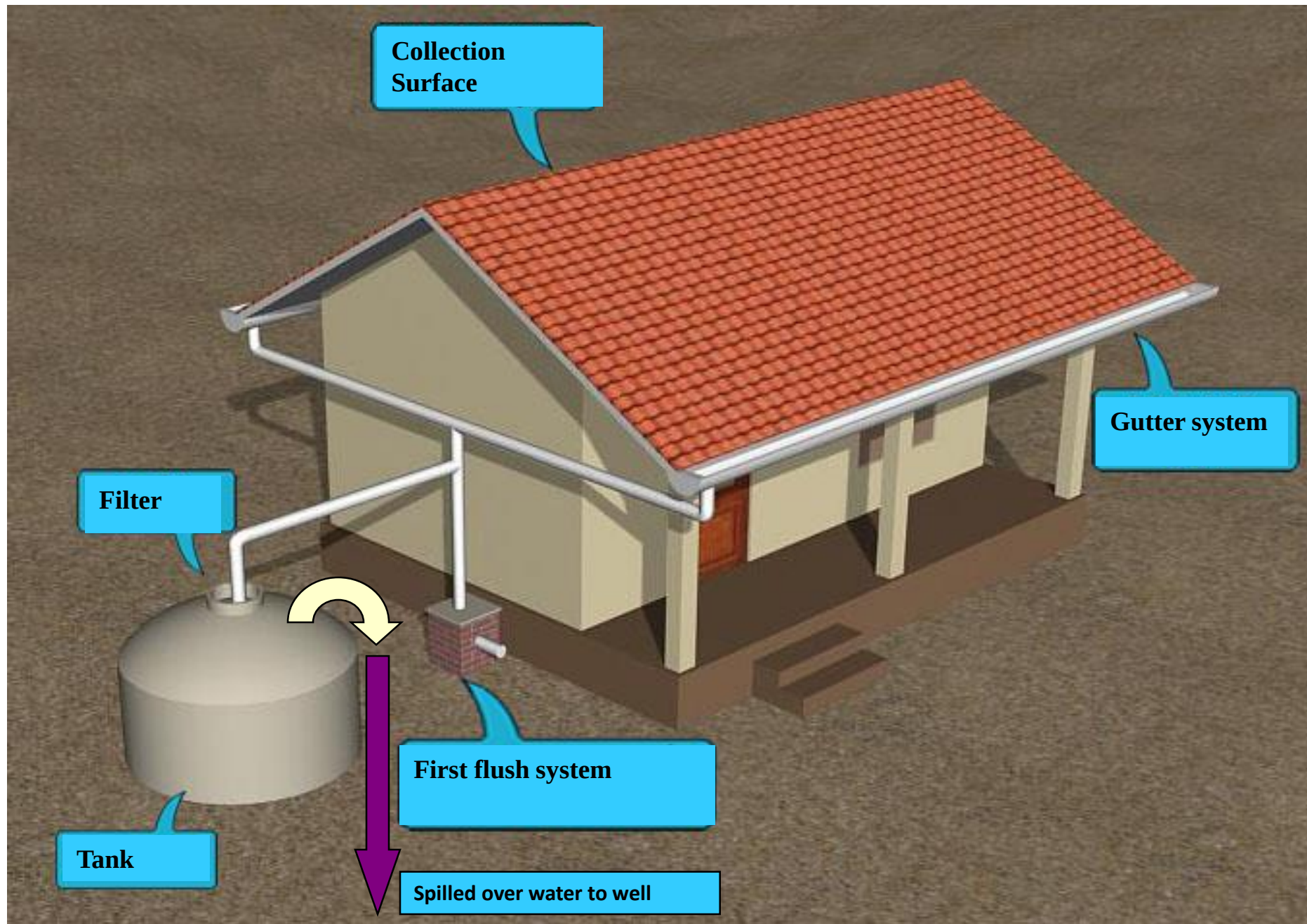
Roof water harvesting system
